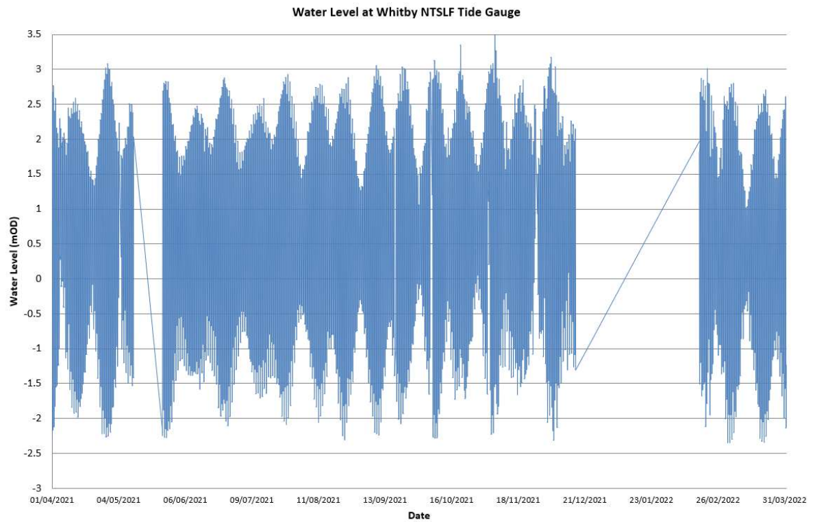
Figure 2.11 Water level data record at Whitby NTSLF tide gauge site for 2021-2022
