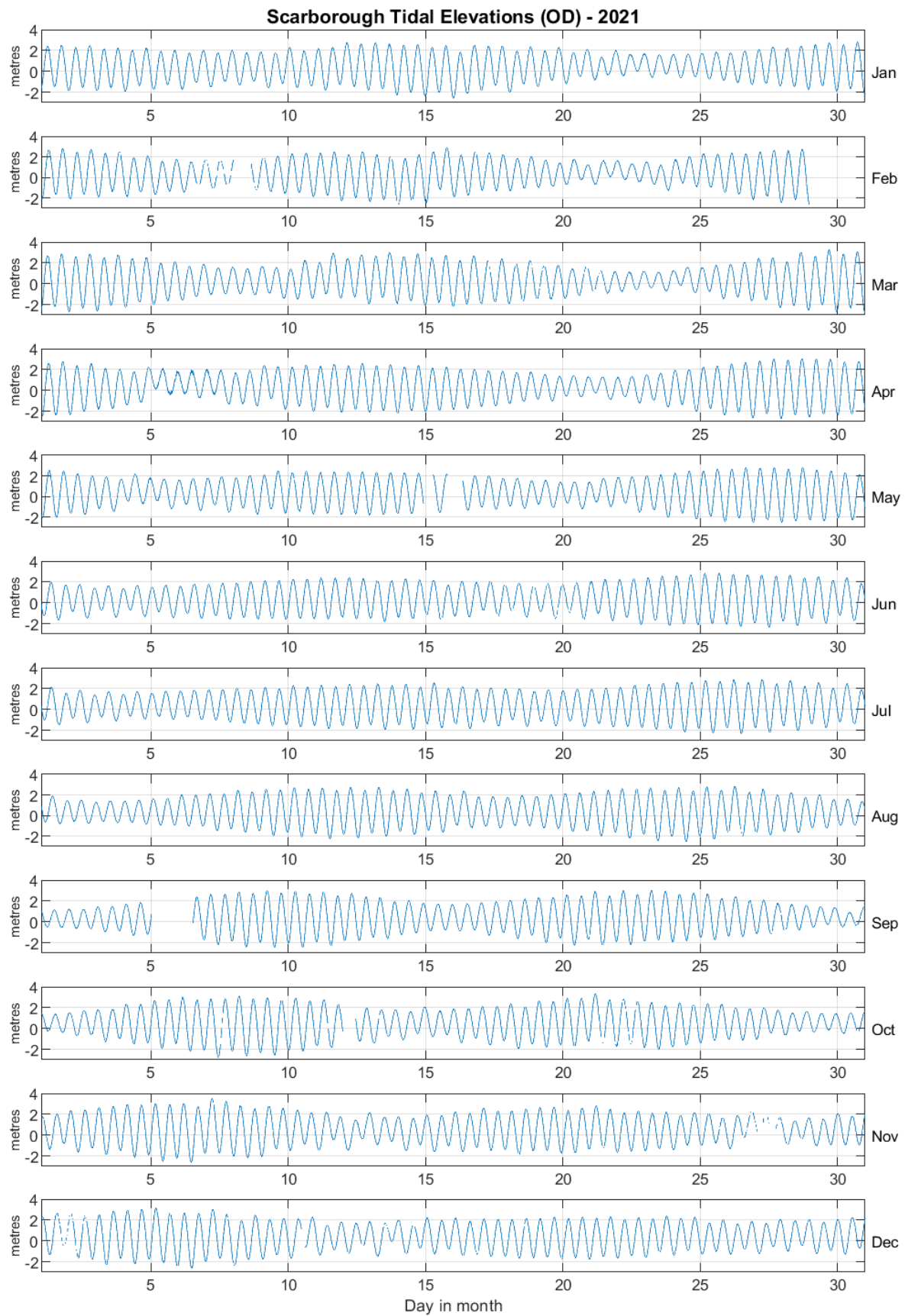
Figure 2: Scarborough tidal elevations for 2021 relative to Ordnance Datum
