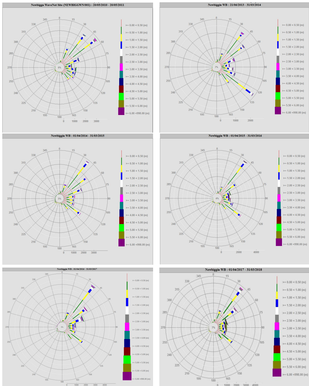
Figure 2.2 Wave roses for Newbiggin WB (original deployment in 2010/11 and subsequent data annually from 2013/14 to date)
