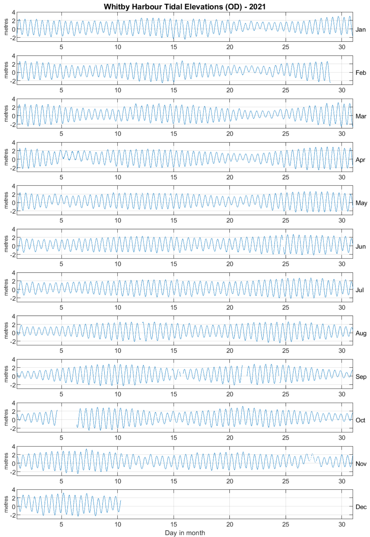
Figure 2: Whitby Harbour tidal elevations for 2021 relative to Ordnance Datum
