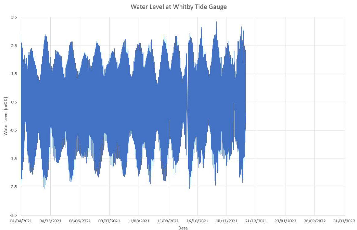
Figure 2.13 Water level data record at Whitby CCO tide gauge site for 2021-2022
