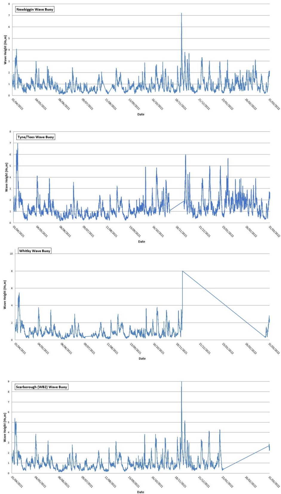
Figure 2.5 Comparison of recorded wave heights at Tyne Tees to the Cell 1 programme buoys from April 2021 to March 2022
