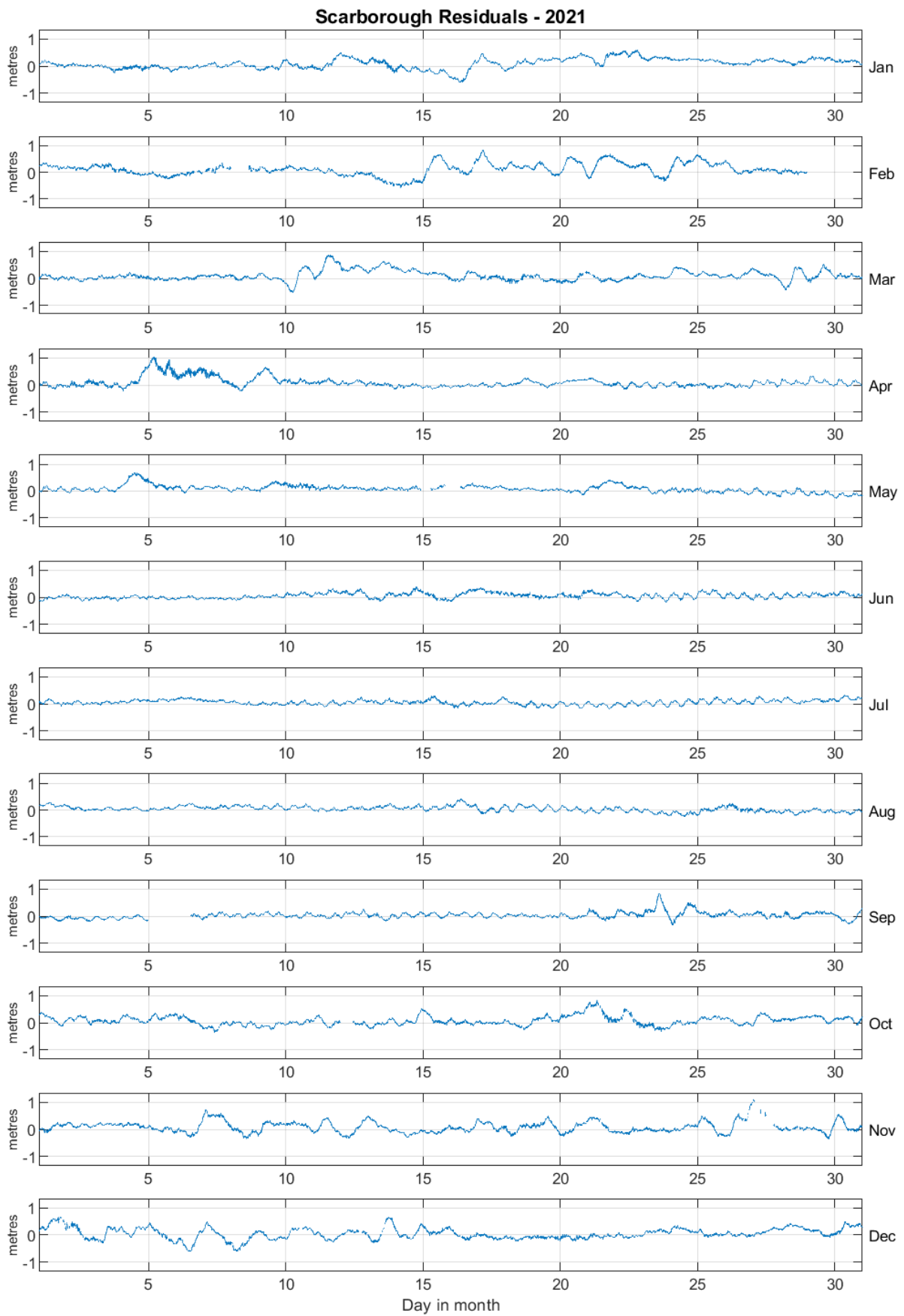
Figure 1: Scarborough residuals for 2021
