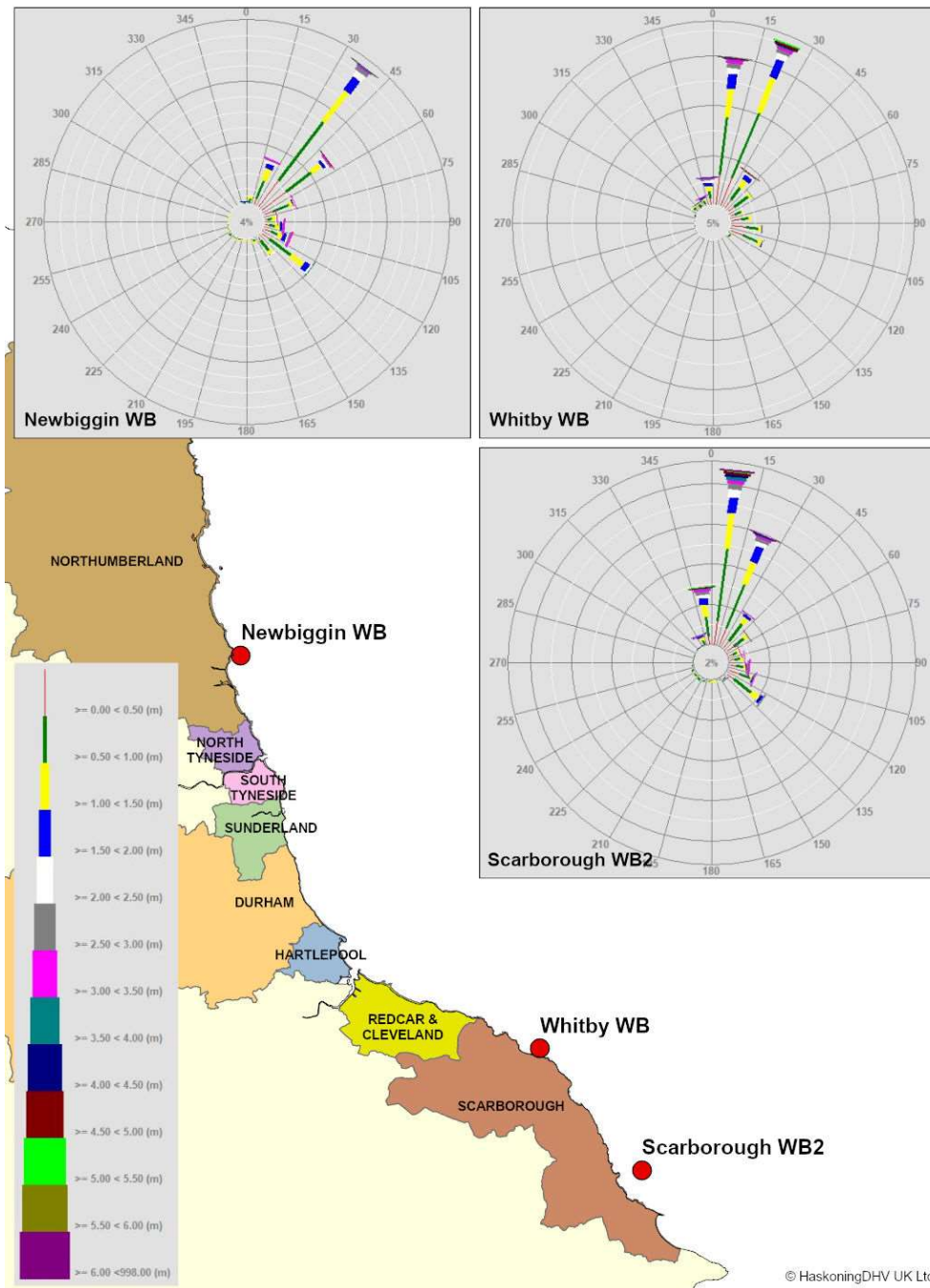
Figure 4.1 Wave Roses (2021/22) from Newbiggin Ness, Whitby and Scarborough
