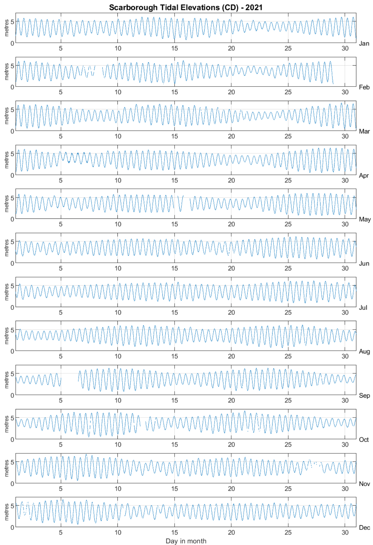
Figure 3: Scarborough tidal elevations for 2021 relative to Chart Datum
