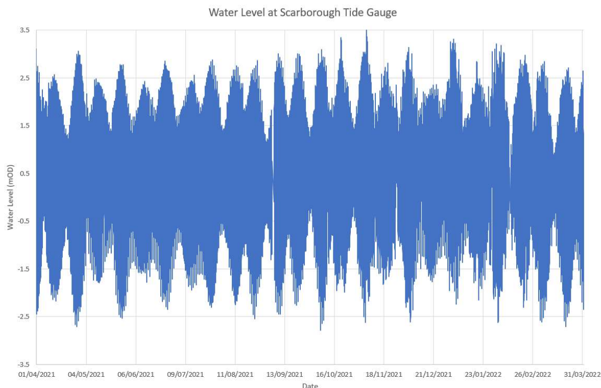
Figure 2.18 Water Levels at Scarborough TG Recorded Tide Site for 2020-21
